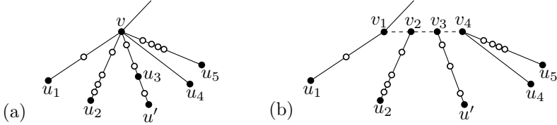
Fig. 2. Transforming the input tree (a) into a rooted tree where each internal vertex has two children (b). The dashed edges in (b) have length zero.
