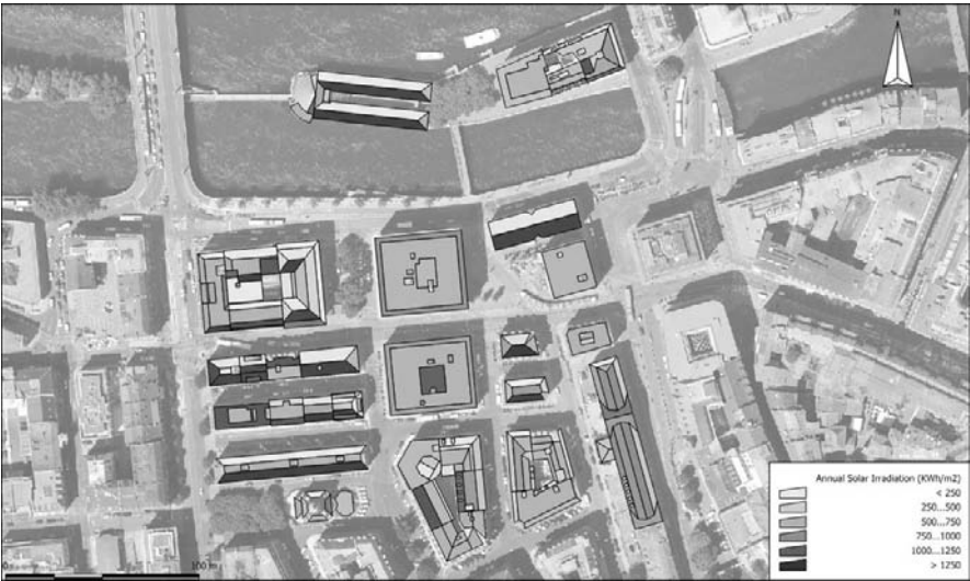
Fig. 17. Annual solar irradiance values (KWh/m 2 ) for the first pilot zone
