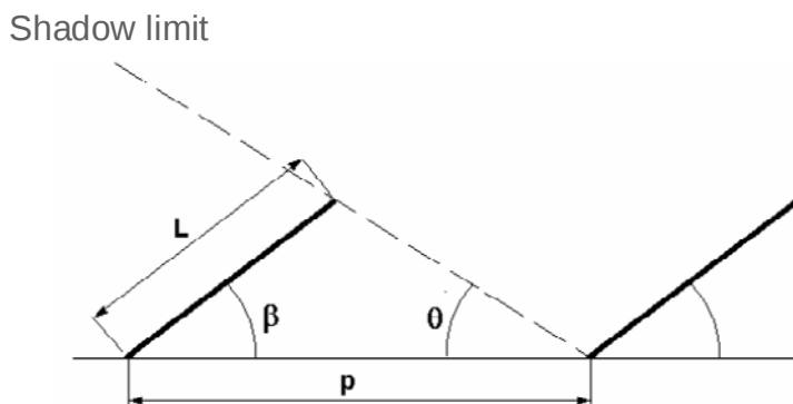
Fig. 7. Implementation of inclined PV panels on flat roof (adapted from PACER, 1996)
