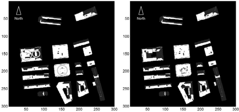
Fig.8. Estimation of suitable areas (in white) and unsuitable roofs (in gray) for the installation of solar panels or PV modules on urban roofs. On the map on the right the authors propose a more restrictive condition, discarding areas where SVF values are smaller than 60%. Hence, areas like terraces facing courtyards or behind chimneys (highlighted with circles) are eliminated
