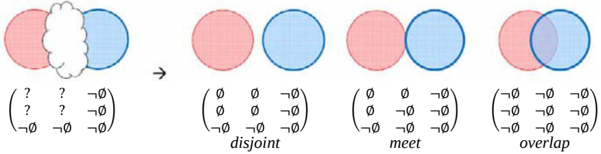
Fig. 5. A 3-9i matrix, which are mapped to three relations in \mathcal{TR}_{\mathbf{RR} - \mathbb{R}^2} by the candidate-listing operation
